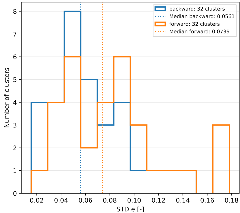
K=32 | Within-cluster STD distributions | Each cluster counts once
